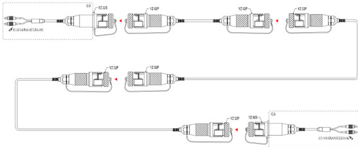
Two equipment Link connection extending Drawing
